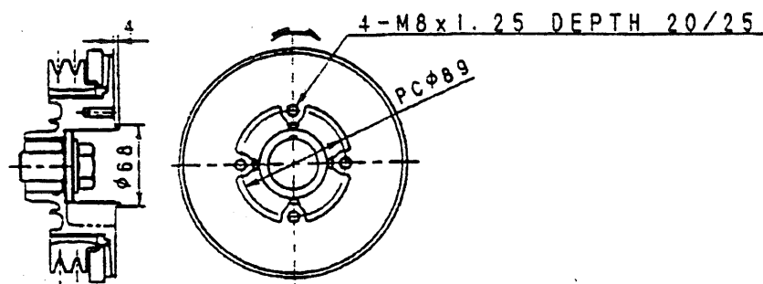
DETAIL OF PULLEY (1/5)
