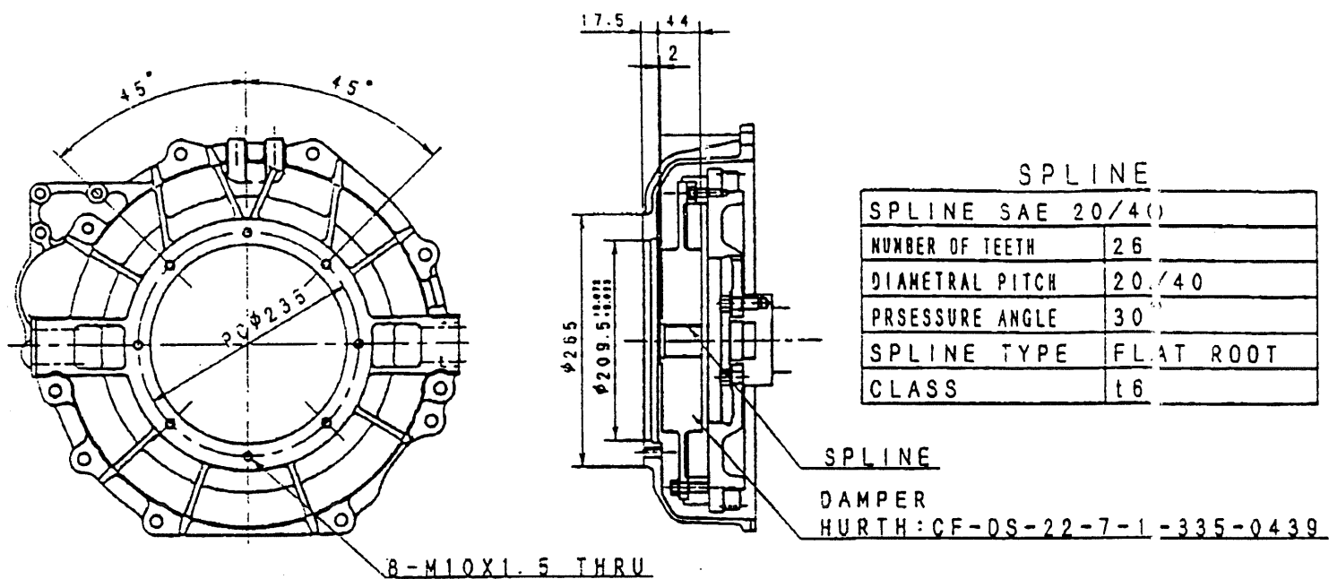
DETAIL OF FLYWHEEL (1/5)
