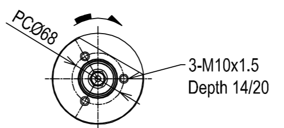
DETAIL OF PULLEY VIEWED FROM A
